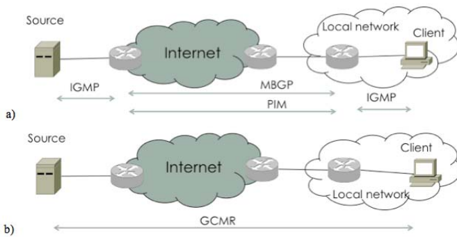
Fig. 1. Protocols architecture a) using PIM-SSM, b) using GCMR
