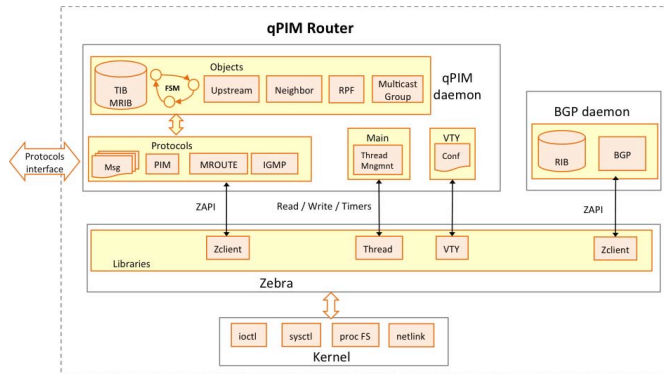
Fig. 3. PIM-SSM node architecture
