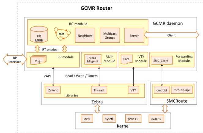
Fig. 2. GCMR node architecture
