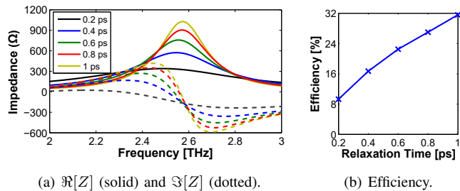
Fig. 5. Resonance characteristics of the graphene dipole as a function of the relaxation time \tau .
